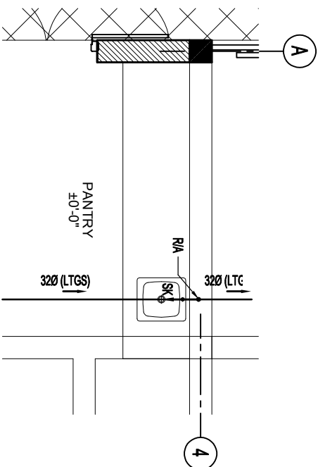
WATER SUPPLY DETAILS SCALE - 1 : 40
